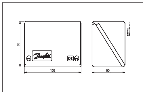
IP55 enclosure
